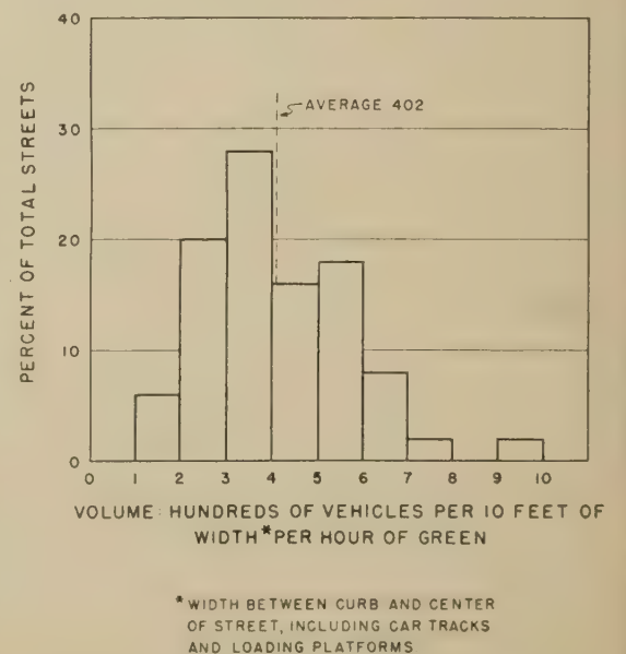
Figure 25.—Frequency distribution of observed intersection capacities on downtown streets with streetcars.
